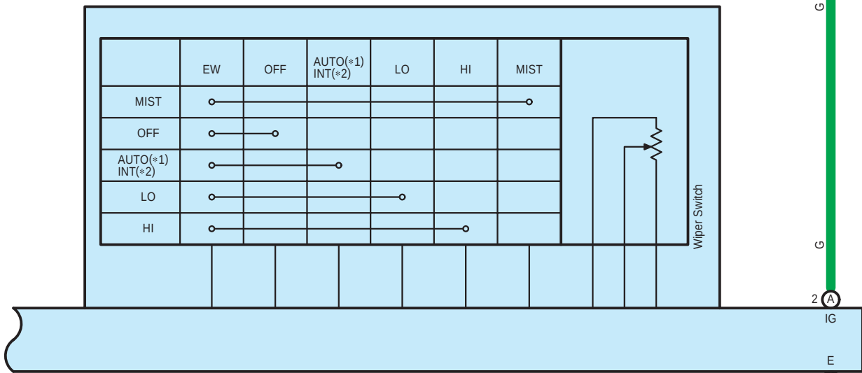
L25(A) Windshield Wiper Switch
